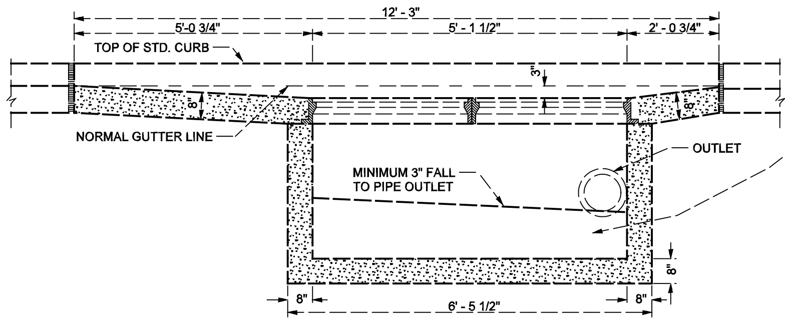
SECTION J - J
