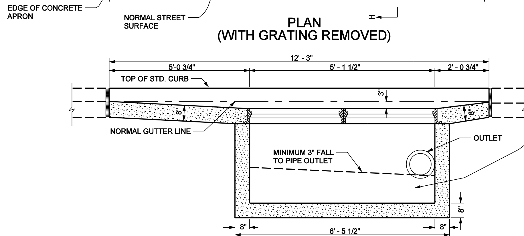
SECTION J - J
