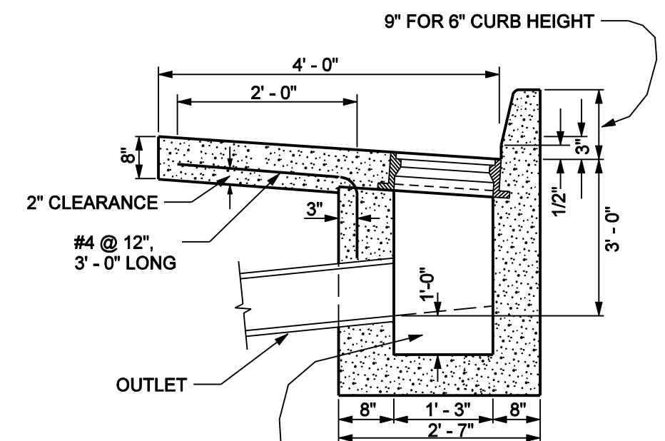
SECTION H - H
