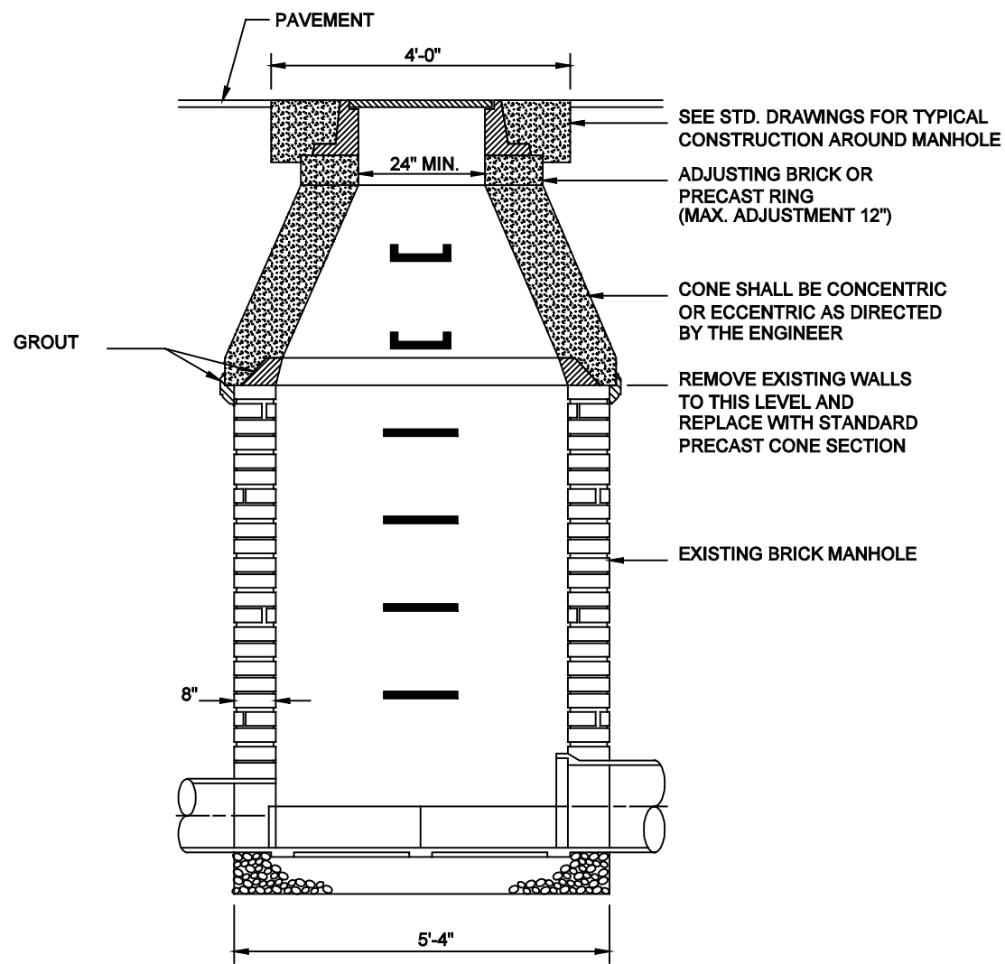
TYPICAL CONSTRUCTION - REBUILDING MANHOLE CONE SECTION
