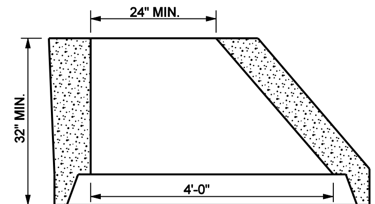
ECCENTRIC CONE
