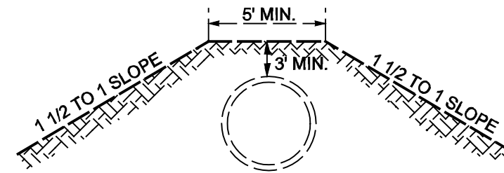
TYPICAL SECTION SEWER IN FILL
